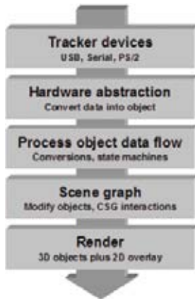
Layering Model of Tinmith
